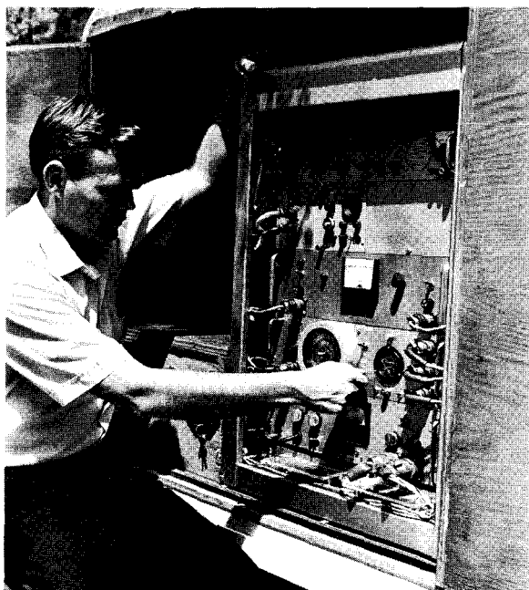
A geophysicist uses trailer-mounted equipment to record micro-earthquakes along the San Andreas fault in California
