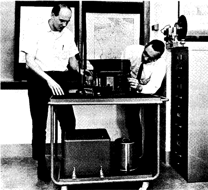
Strong-motion accelerograph for earthquake studies to be installed in Caltech's Millikan Library building
